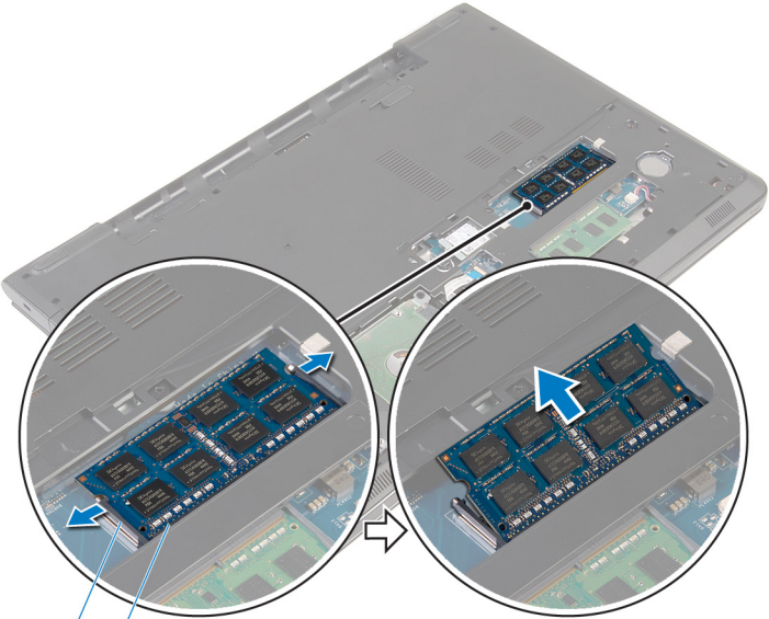
1 2 1 securing clips (2)
